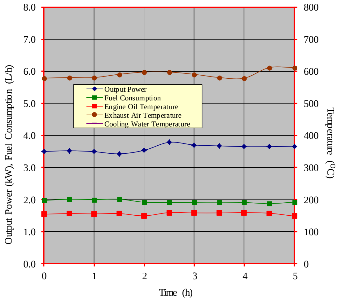
Figure 4. Performance characteristic curves during the continuous running test of the DORADO DJ168F gasoline engine
