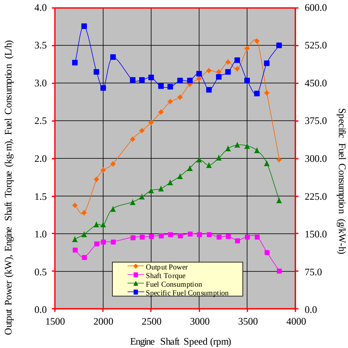
Figure 3. Performance characteristic curves of the DORADO DJ168F gasoline engine
